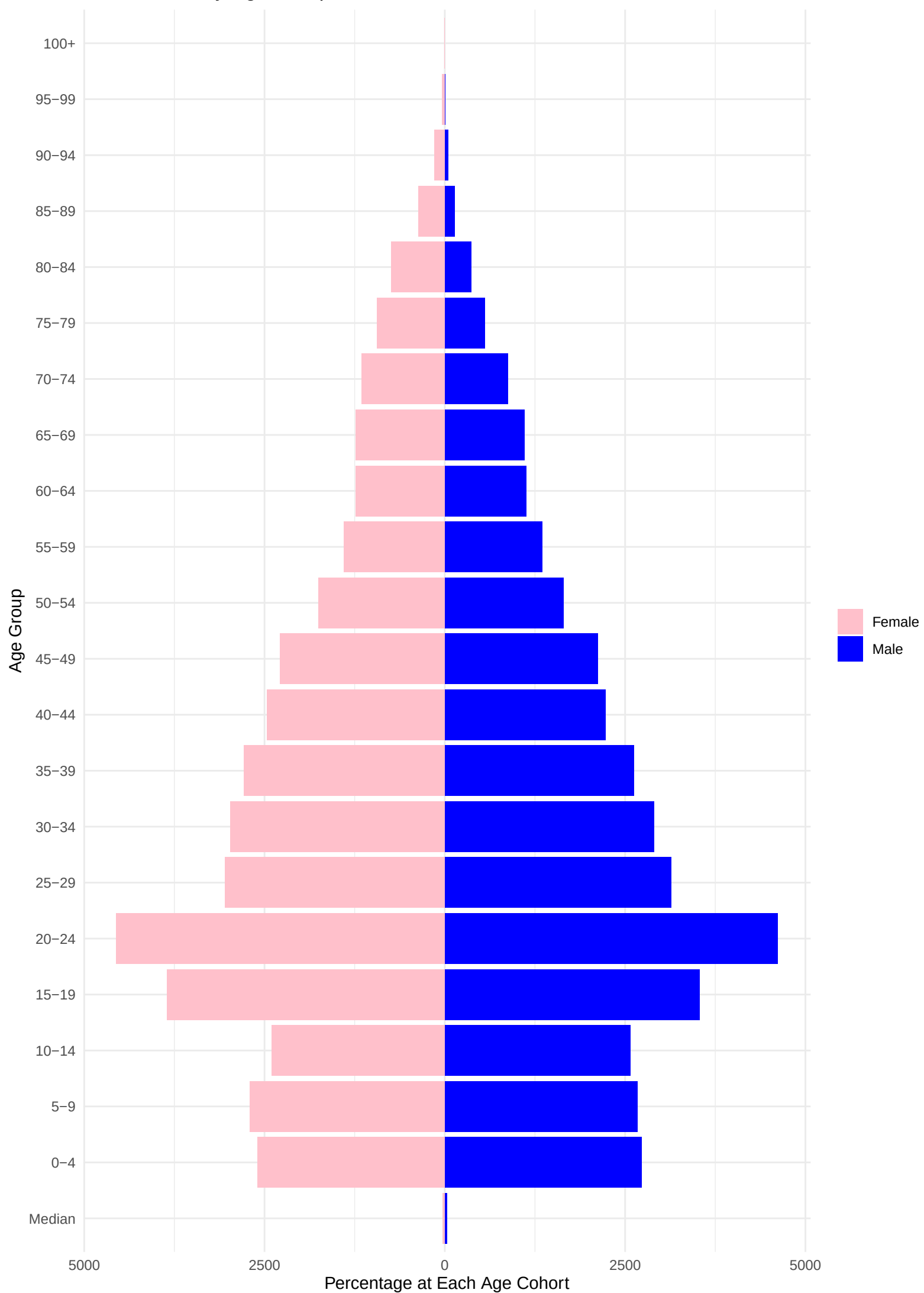
Tornado Plot by Age Group, Year: 1996 Area: Palmerston North
